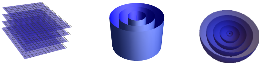
Figure 2.1: Level sets of the isoparametric function f_k: \mathbb{R}^3 \rightarrow \mathbb{R} , defined by f_k(x_1, x_2, x_3) := \sum_{i=1}^k x_i^2 , for each k \in \{1, 2, 3\} , respectively.
