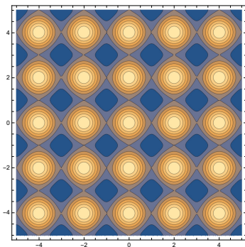
Figure 2.7: Level sets of h on \mathbb{R}^2 .
