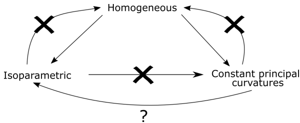
Figure 2.6: Hypersurfaces in \mathbb{H}H^n and \mathbb{O}H^2 .
