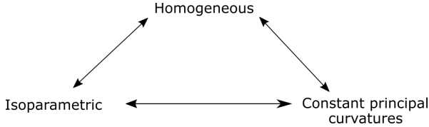
Figure 2.2: Hypersurfaces in \mathbb{R}^n and \mathbb{R}H^n .
