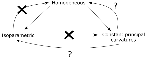
Figure 2.4: Hypersurfaces in \mathbb{C}P^n and \mathbb{C}H^n .
