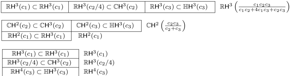
Figure 6.1: Three examples of Young tableaux adapted to the product M = \mathbb{R}\mathbb{H}^3(c_1) \times \mathbb{C}\mathbb{H}^3(c_2) \times \mathbb{H}\mathbb{H}^3(c_3) , along with the irreducible factors of the corresponding totally geodesic submanifolds presented at the end of each row (see Proposition 6.2.12). Notice that the isometry type of these totally geodesic submanifolds can be computed using Corollary 6.2.11.
