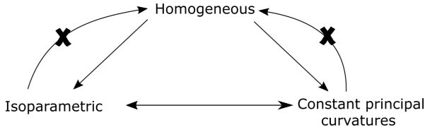
Figure 2.3: Hypersurfaces in S^n .
