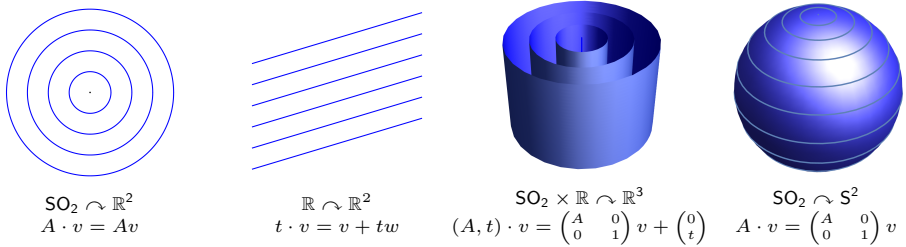
Figure 3.1: Examples of cohomogeneity one actions.
