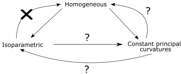
Figure 2.5: Hypersurfaces in \mathbb{H}P^n .
